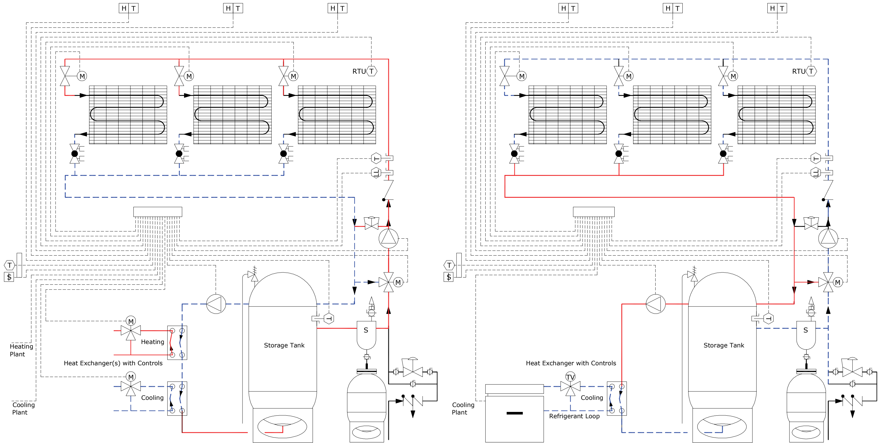
Heating/Cooling Heat Exchangers with Storage Tank for Radiant Ceiling Systems
